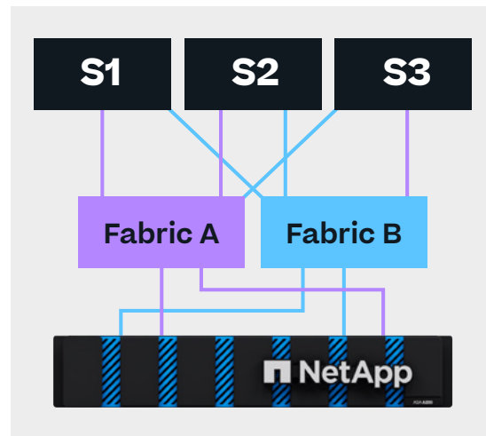
Figure 1) Symmetric active-active topology.
