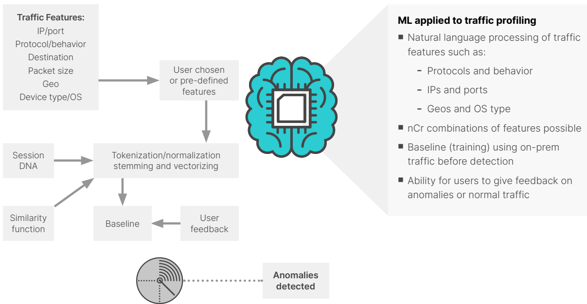
Figure 3: FortiNDR and ML applications for traffic profiling
