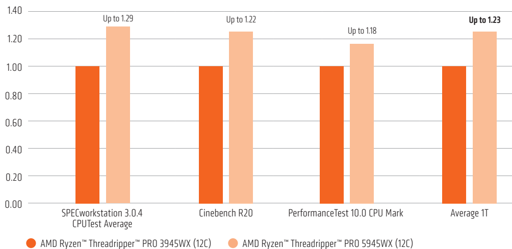
FIGURE 7: MULTI-THREAD (MT) GENERATION-TO-GENERATION 12C TEST RESULTS FOR SIMILARLY CONFIGURED SYSTEMS 5,6 , NORMALIZED TO AMD THREADRIPPER PRO 3945WX
