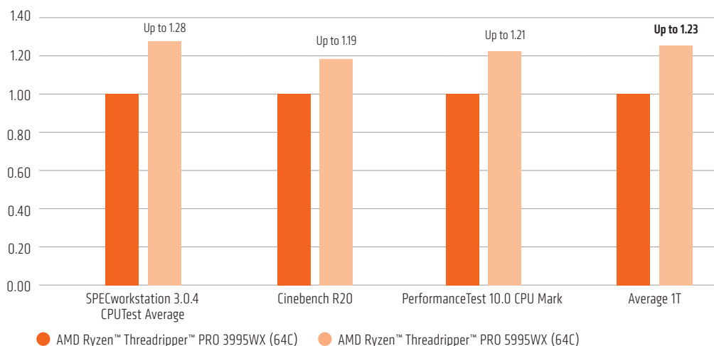
FIGURE 8: MULTI-THREAD (MT) GENERATION-TO-GENERATION 64C TEST RESULTS FOR SIMILARLY CONFIGURED SYSTEMS 5,6 , NORMALIZED TO AMD THREADRIPPER PRO 3995WX
