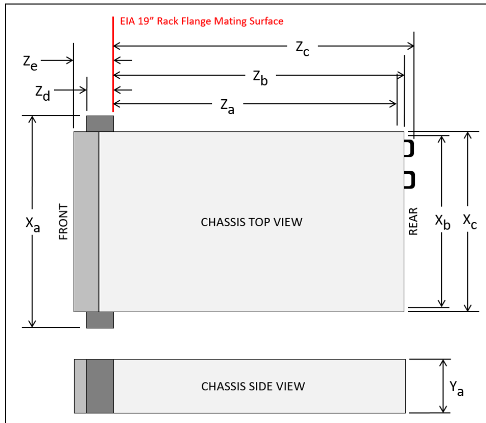
Figure 15. Server dimensions
