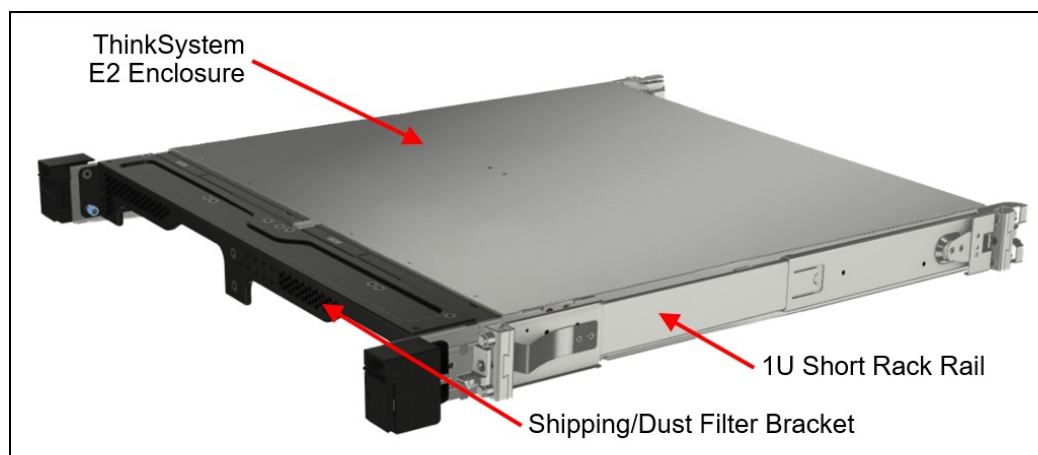
Figure 28. ThinkSystem E2 Enclosure with a short rail kit (rail in closed position)
